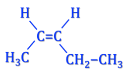
cis-2-penteno
